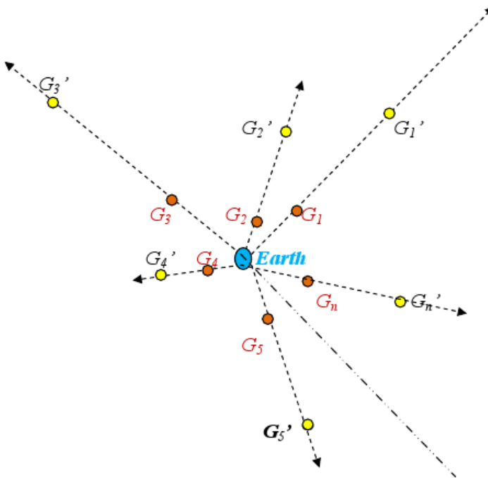
Fig. 31. Diagram of Allegedly Expansion Universe
