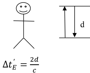
Fig. 18. Observer on Earth
