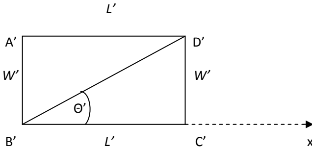
Fig. 3. Contracted Lengths of the Rectangular Object Moving Along the x-Axis
