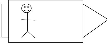
Fig. 19. Observer in the Rocket
