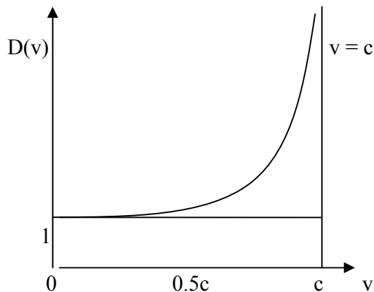
Fig. 1. The Graph of the Time-Dilation Factor
