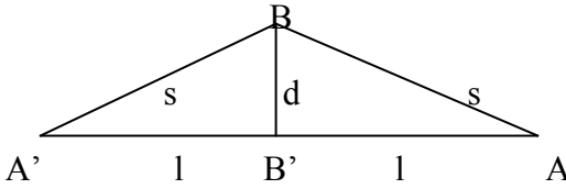
Fig. 20. Computing the Elapsed Time
