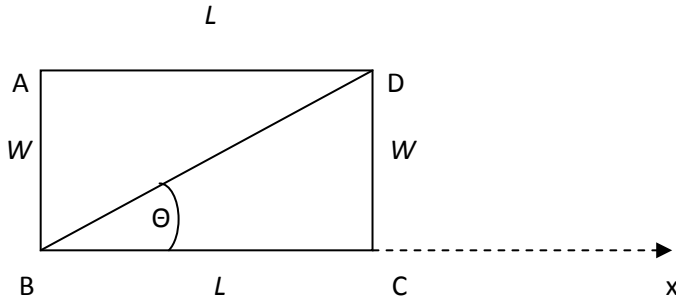
Fig. 2. A Rectangular Object Moving Along the x-Axis
