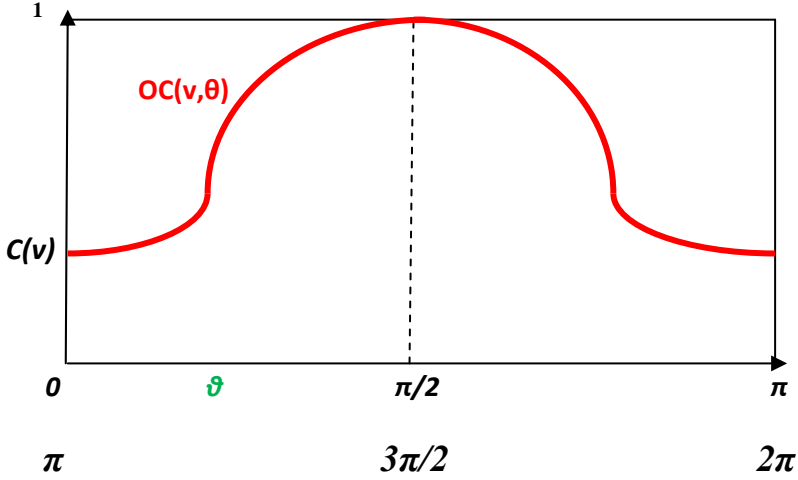
Fig. 4. The Graph of the Oblique-Length Contraction Factor OC(v, \theta)
