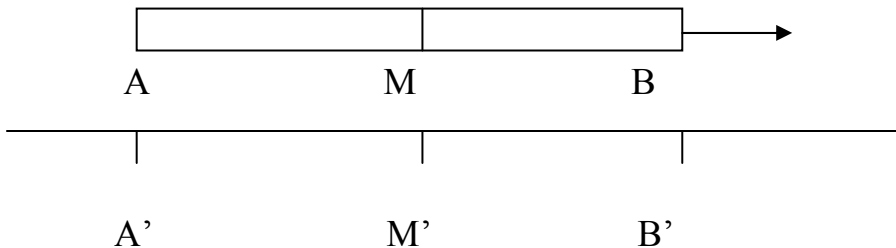
Fig. 21. The Paradox of Simultaneity
